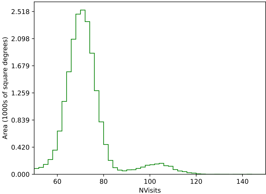
ddf_acor_sf10_lsf20_lsr50_v3.4_10yrs All sky g band: NVisits
