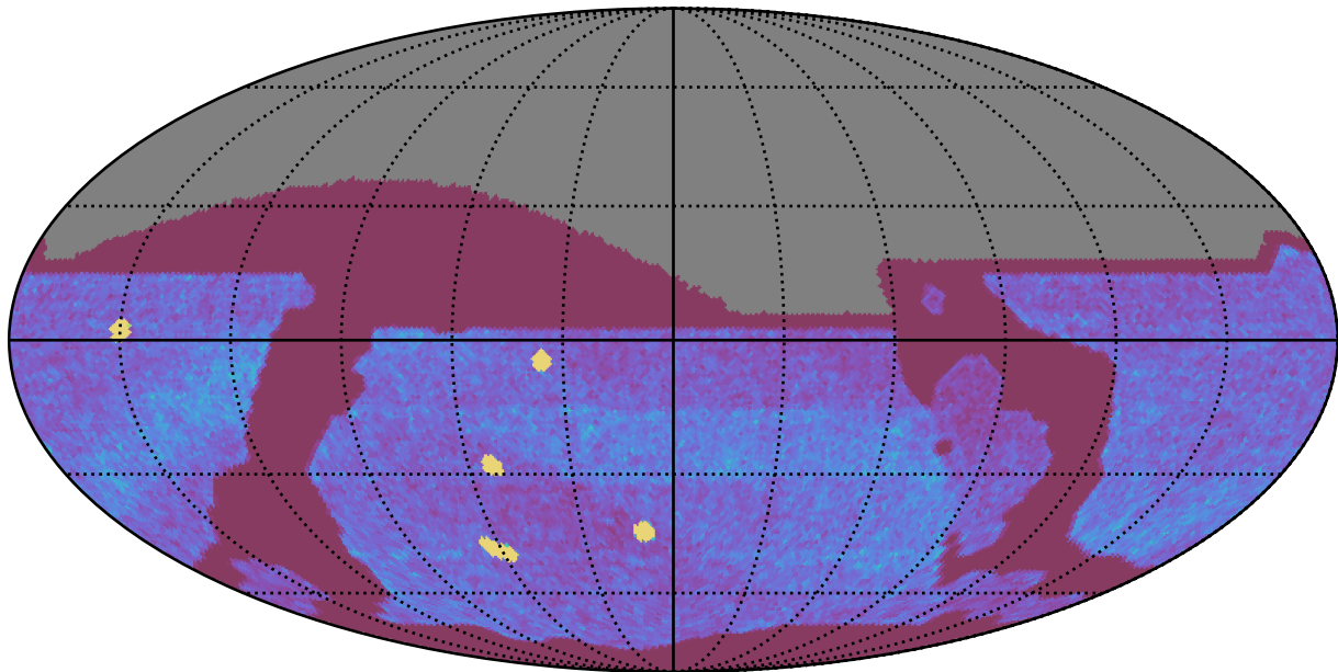
ddf_acor_sf10_lsf20_lsr50_v3.4_10yrs All sky all bands: NVisits
