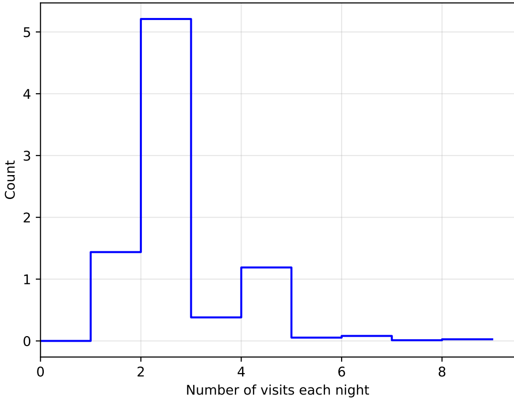
ddf_acor_sf10_lsf20_lsr50_v3.4_10yrs WFD: NVisitsPerNight 1e6
