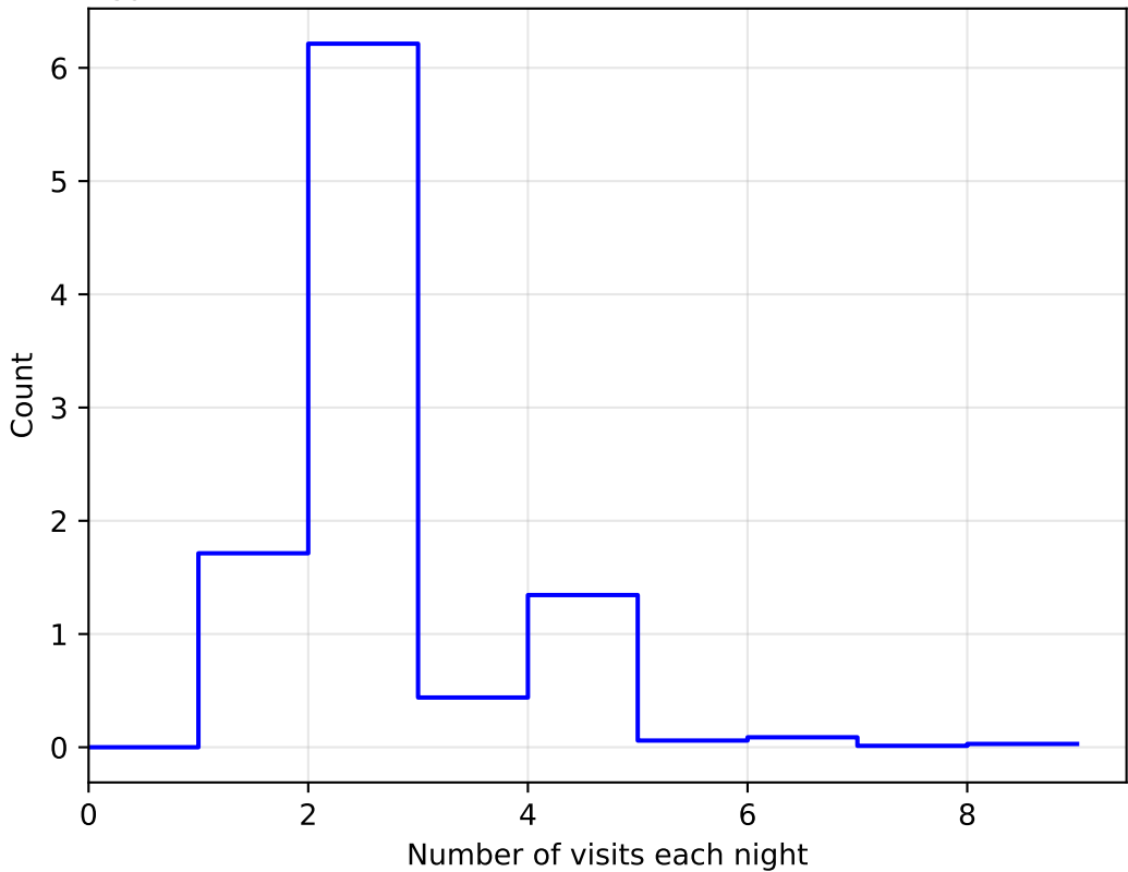
ddf_acor_sf10_lsf20_lsr50_v3.4_10yrs All sky: NVisitsPerNight 1e6
