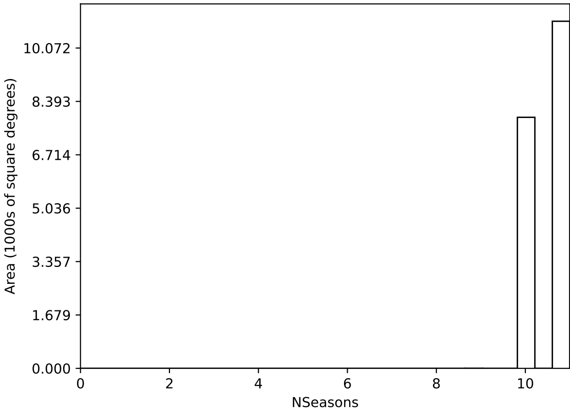
ddf_acor_sf10_lsf20_lsr50_v3.4_10yrs WFD all bands: NSeasons
