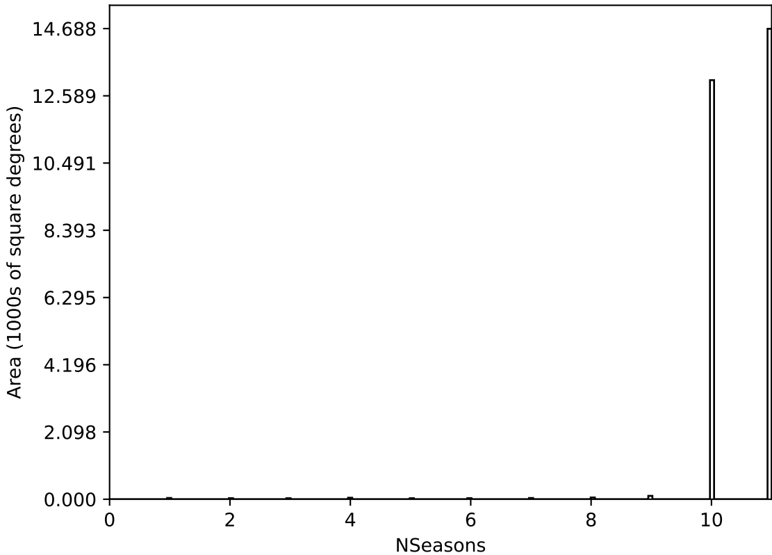
ddf_acor_sf10_lsf20_lsr50_v3.4_10yrs All sky all bands: NSeasons
