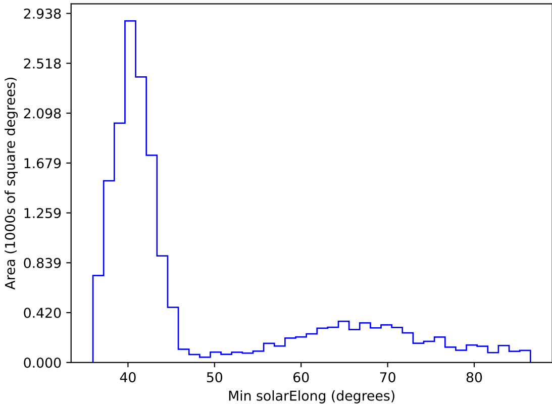
ddf_acor_sf10_lsf20_lsr50_v3.4_10yrs WFD z band: Min solarElong
