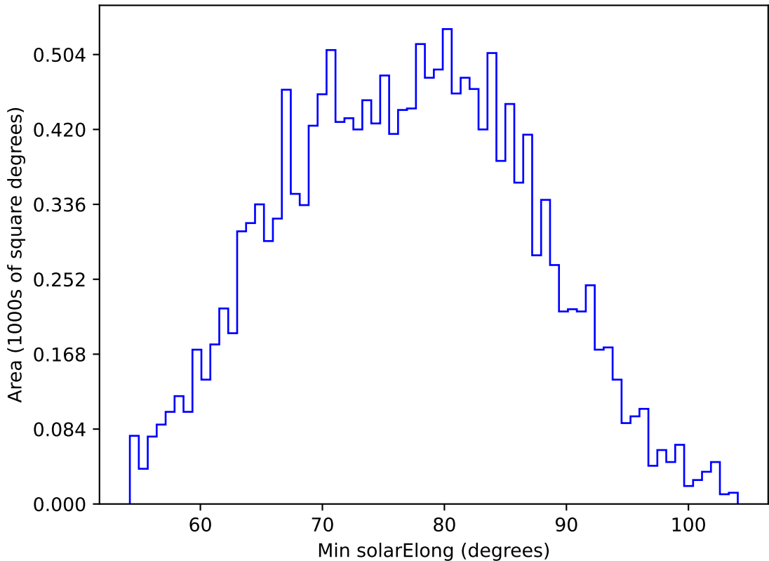
ddf_acor_sf10_lsf20_lsr50_v3.4_10yrs WFD u band: Min solarElong
