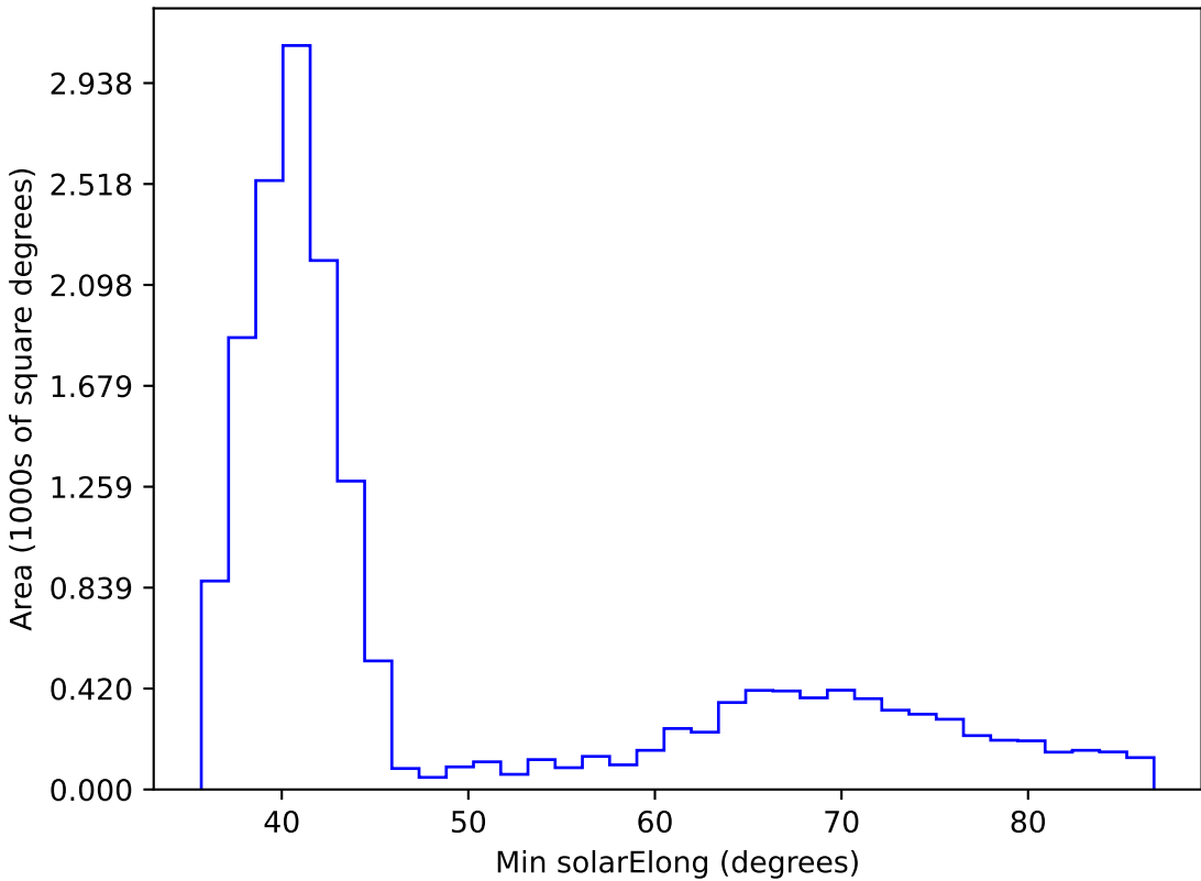
ddf_acor_sf10_lsf20_lsr50_v3.4_10yrs WFD i band: Min solarElong
