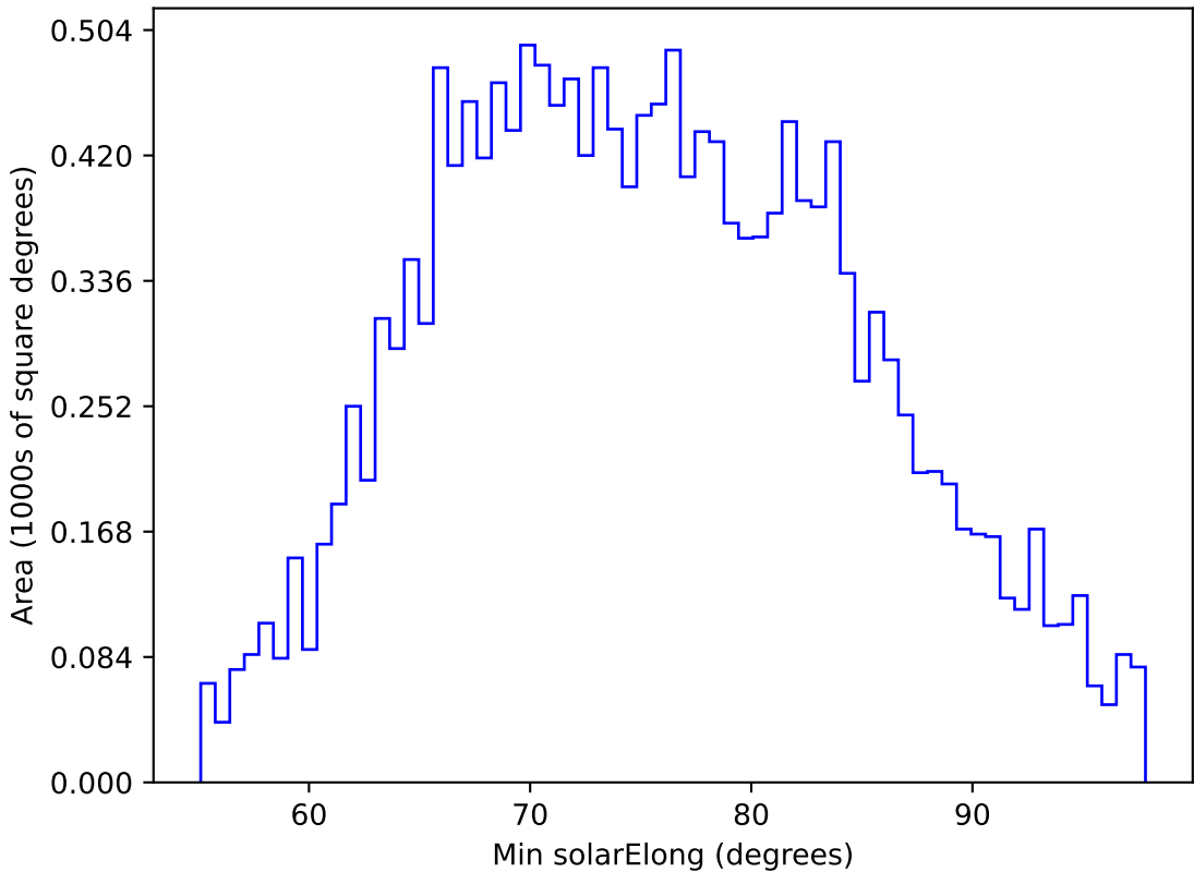
ddf_acor_sf10_lsf20_lsr50_v3.4_10yrs WFD g band: Min solarElong
