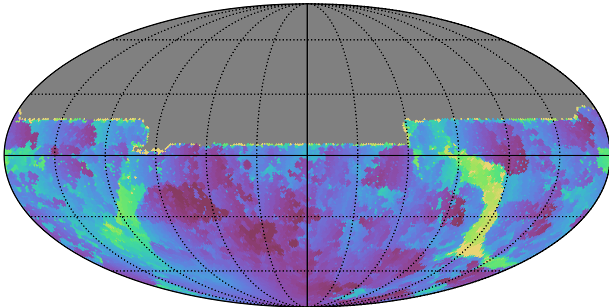
ddf_acor_sf10_lsf20_lsr50_v3.4_10yrs All sky u band: Min solarElong
