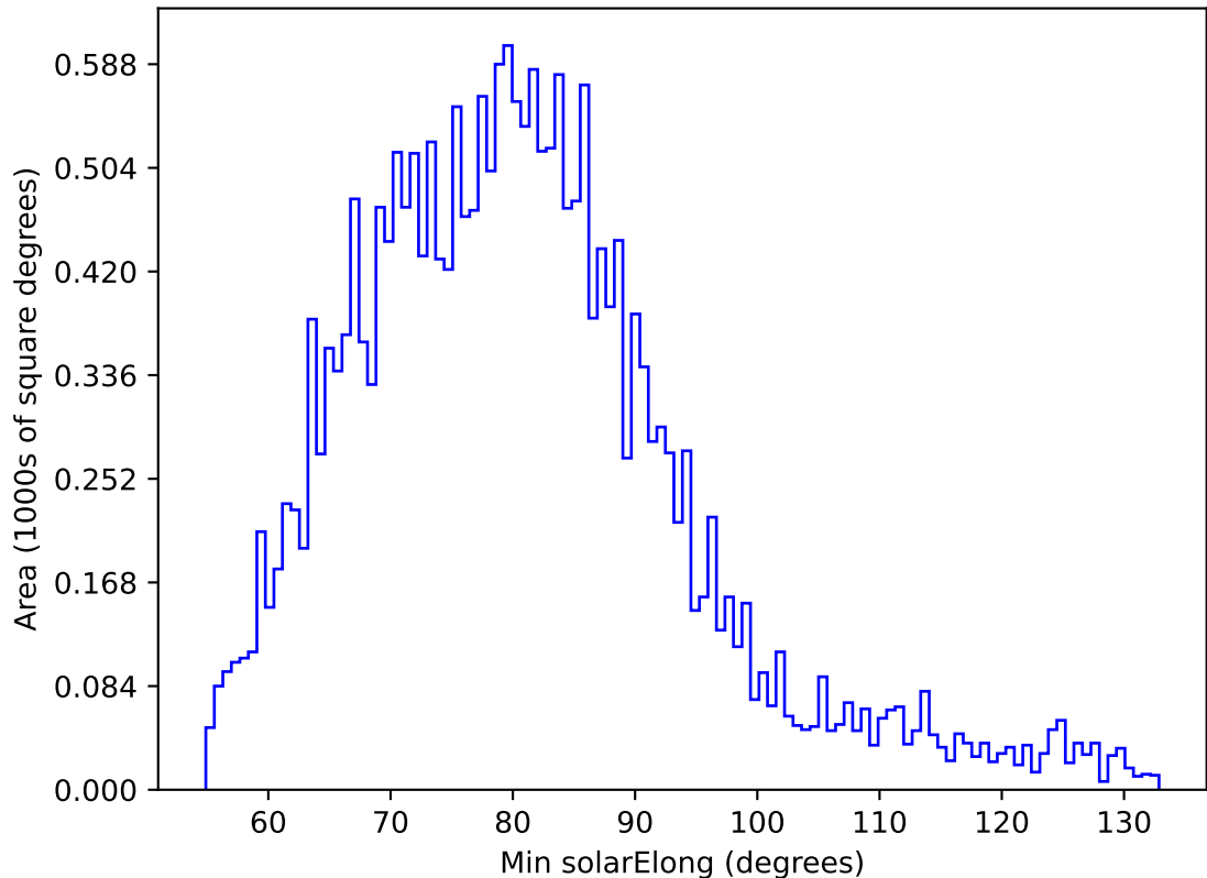
ddf_acor_sf10_lsf20_lsr50_v3.4_10yrs All sky u band: Min solarElong
