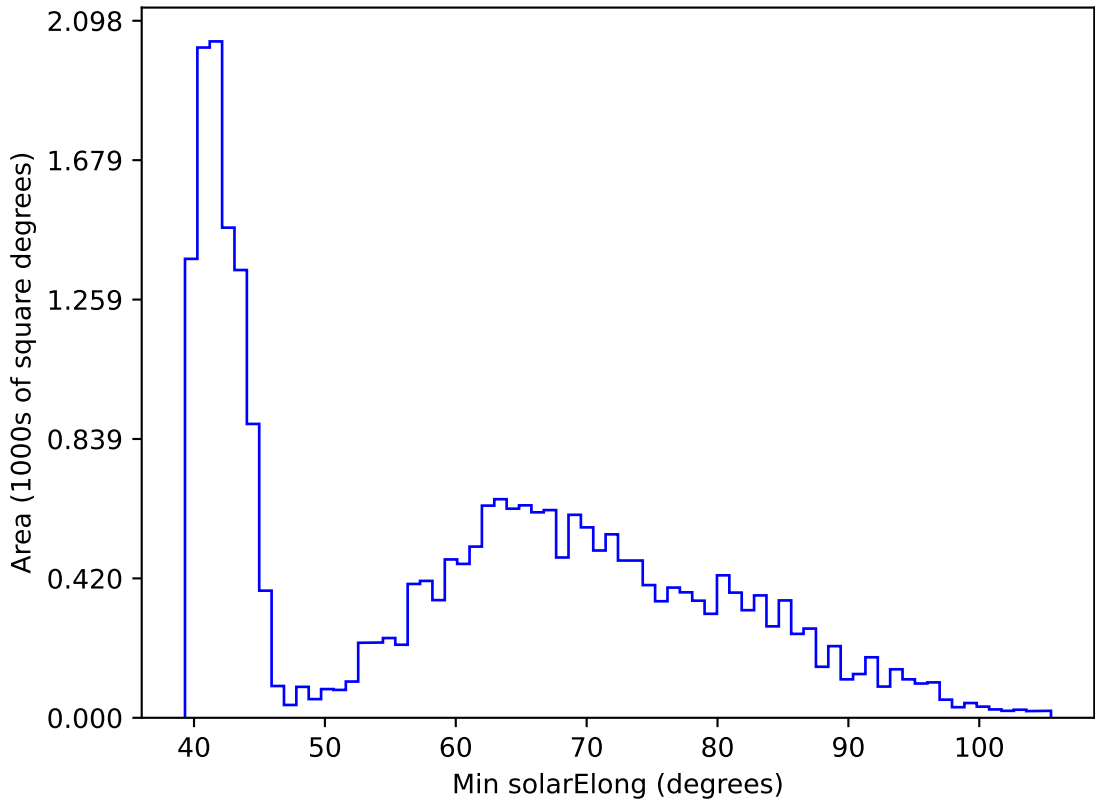
ddf_acor_sf10_lsf20_lsr50_v3.4_10yrs All sky r band: Min solarElong
