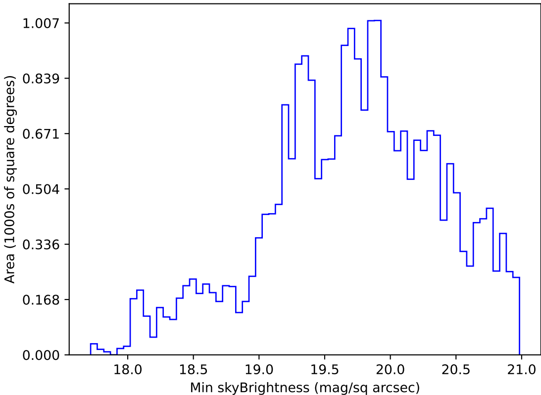
ddf_acor_sf10_lsf20_lsr50_v3.4_10yrs Yr 1 r band: Min skyBrightness
