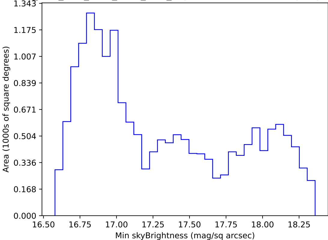
ddf_acor_sf10_lsf20_lsr50_v3.4_10yrs WFD z band: Min skyBrightness
