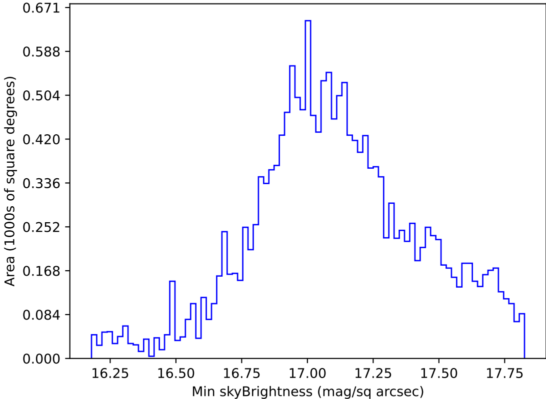
ddf_acor_sf10_lsf20_lsr50_v3.4_10yrs WFD y band: Min skyBrightness
