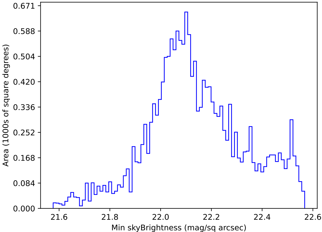
ddf_acor_sf10_lsf20_lsr50_v3.4_10yrs WFD u band: Min skyBrightness
