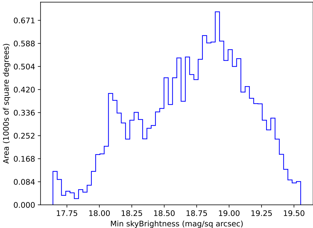
ddf_acor_sf10_lsf20_lsr50_v3.4_10yrs WFD r band: Min skyBrightness
