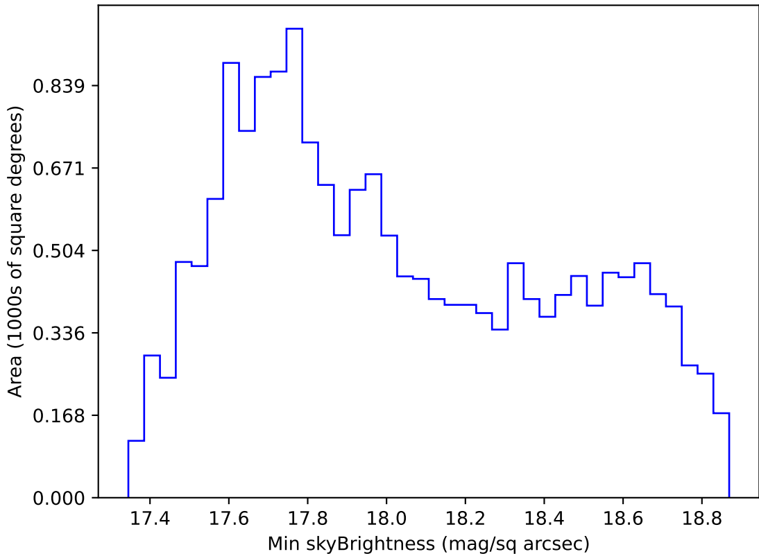
ddf_acor_sf10_lsf20_lsr50_v3.4_10yrs WFD i band: Min skyBrightness
