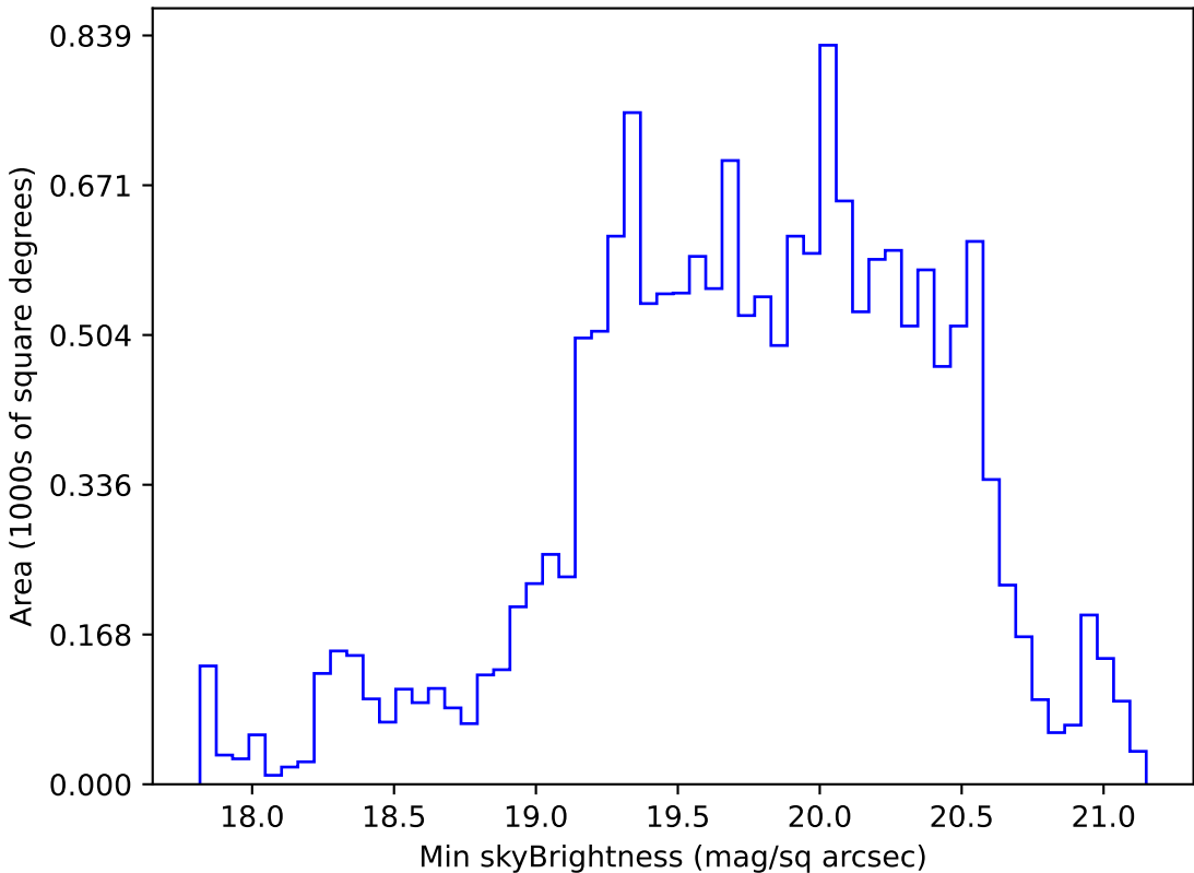
ddf_acor_sf10_lsf20_lsr50_v3.4_10yrs WFD g band: Min skyBrightness
