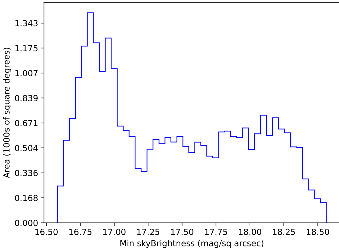
ddf_acor_sf10_lsf20_lsr50_v3.4_10yrs All sky z band: Min skyBrightness
