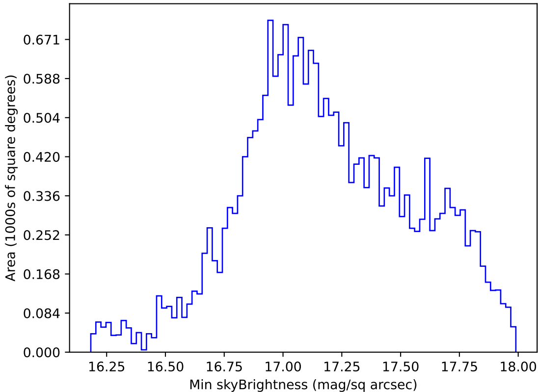
ddf_acor_sf10_lsf20_lsr50_v3.4_10yrs All sky y band: Min skyBrightness
