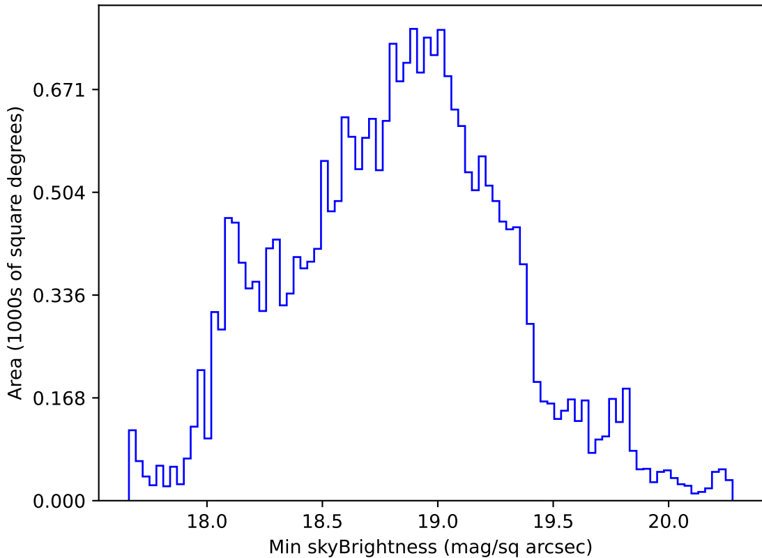
ddf_acor_sf10_lsf20_lsr50_v3.4_10yrs All sky r band: Min skyBrightness
