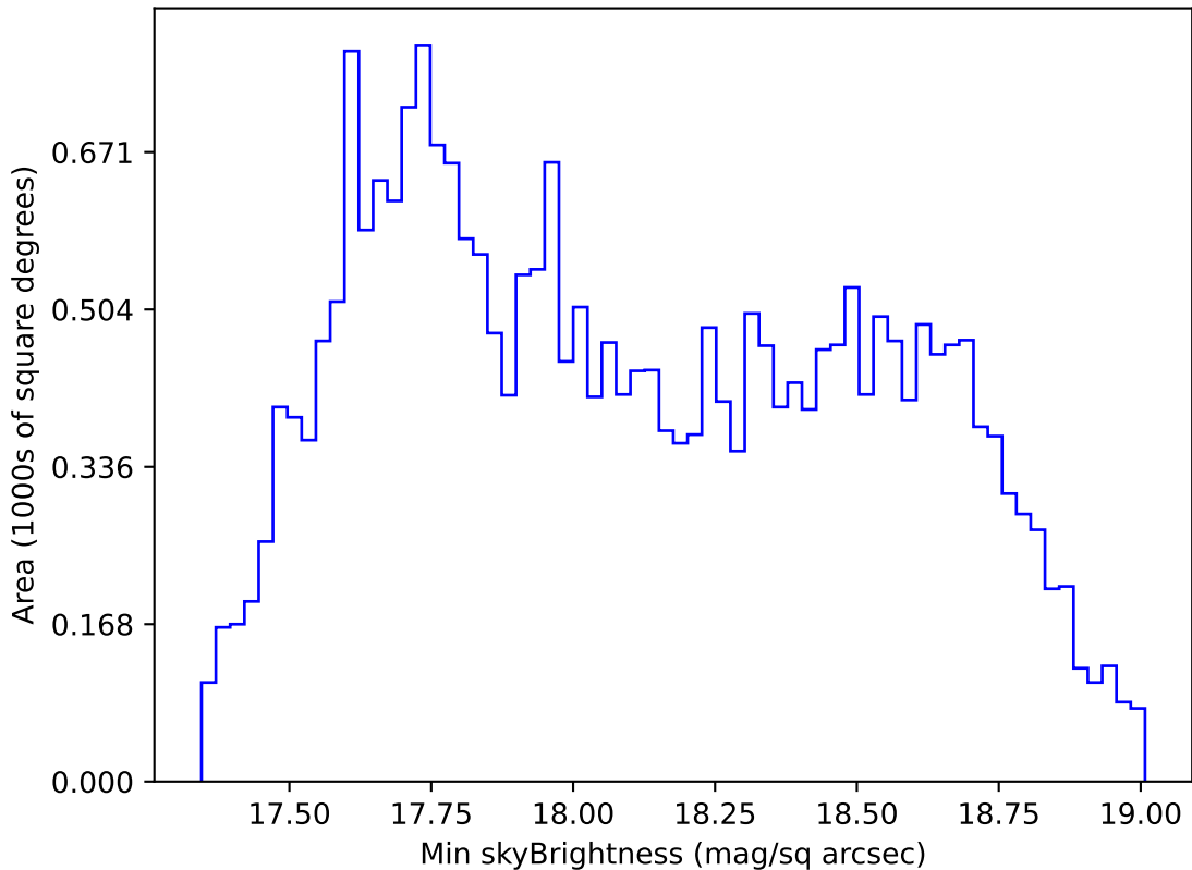
ddf_acor_sf10_ls20_lsr50_v3.4_10yrs All sky i band: Min skyBrightness
