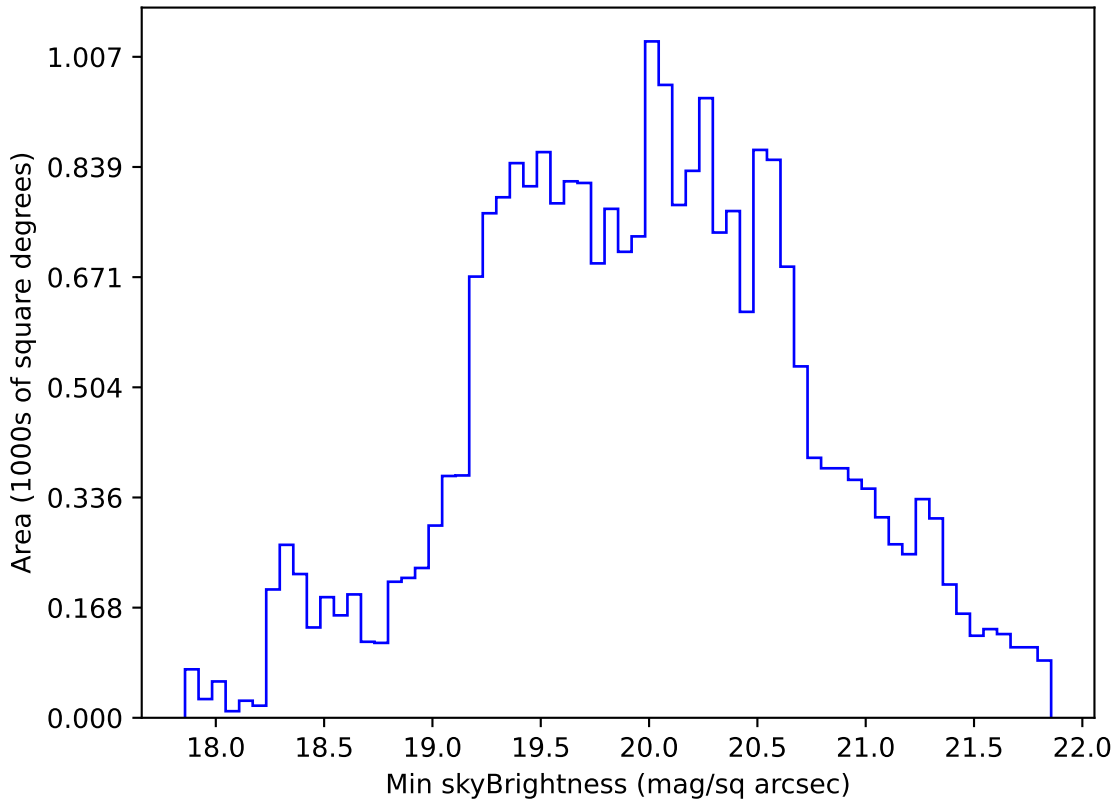
ddf_acor_sf10_lsf20_lsr50_v3.4_10yrs All sky g band: Min skyBrightness
