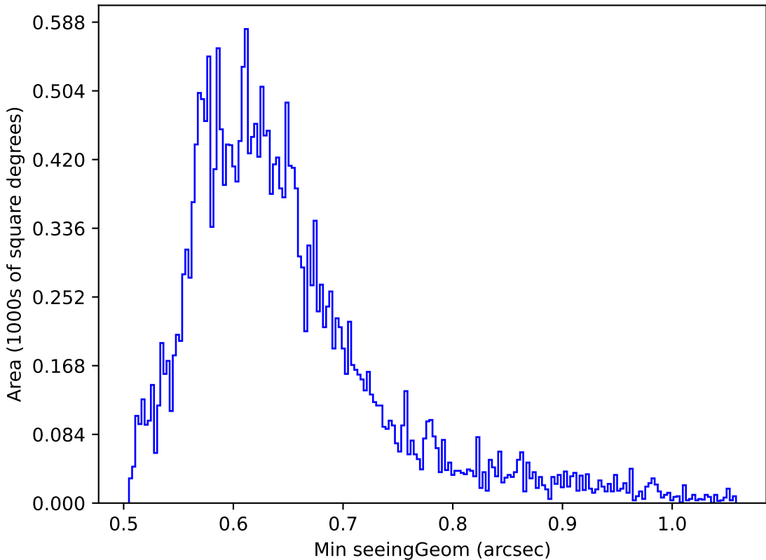
ddf_acor_sf10_lsf20_lsr50_v3.4_10yrs Yr 1 z band: Min seeingGeom
