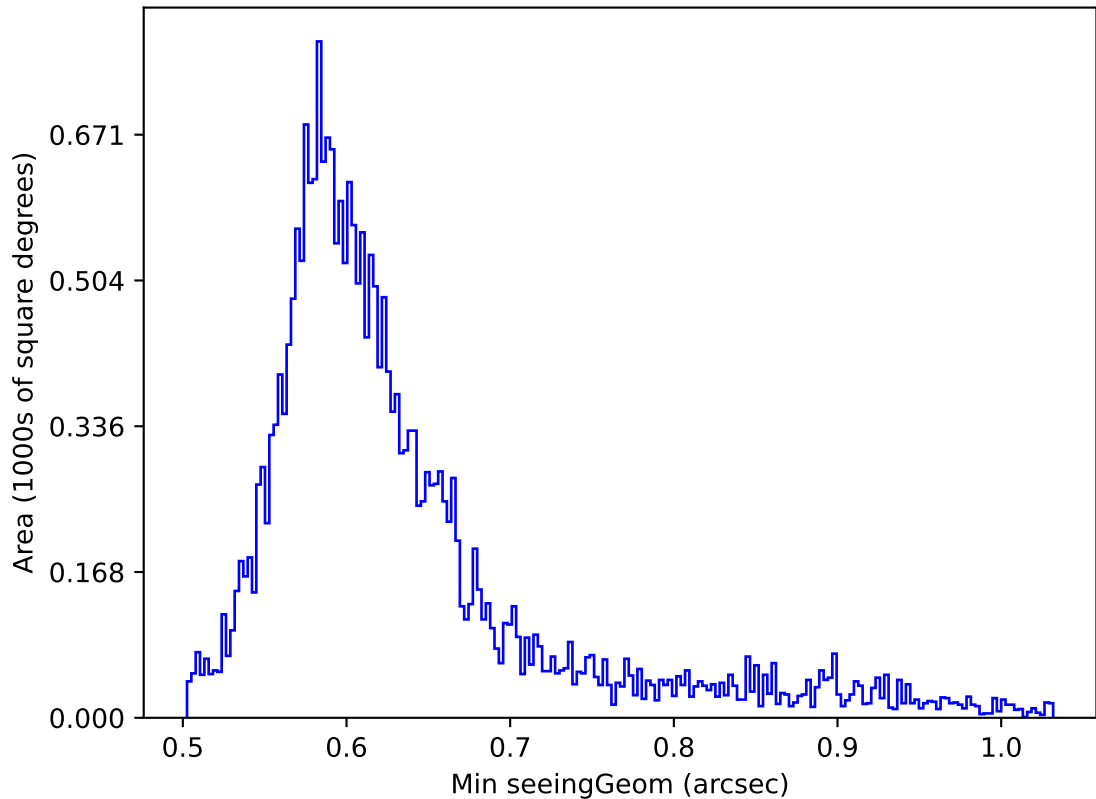
ddf_acor_sf10_lsf20_lsr50_v3.4_10yrs Yr 1 i band: Min seeingGeom
