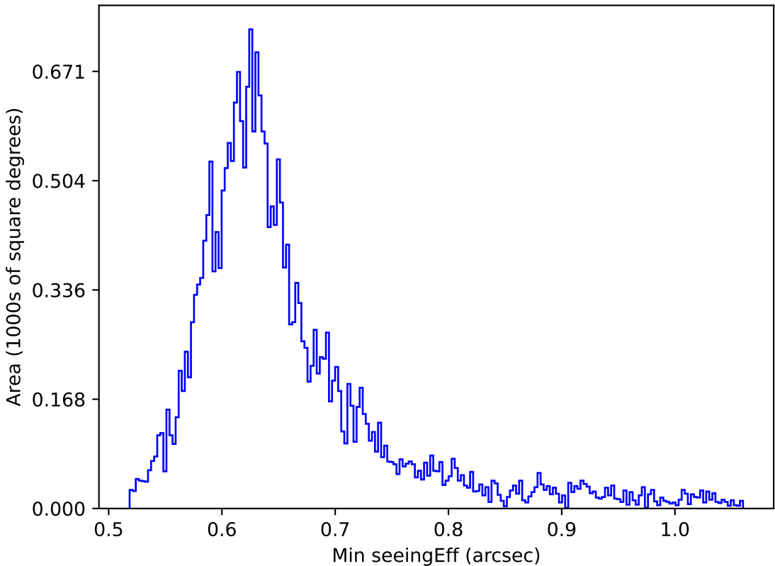
ddf_acor_sf10_lsf20_lsr50_v3.4_10yrs Yr 1 all bands: Min seeingEff
