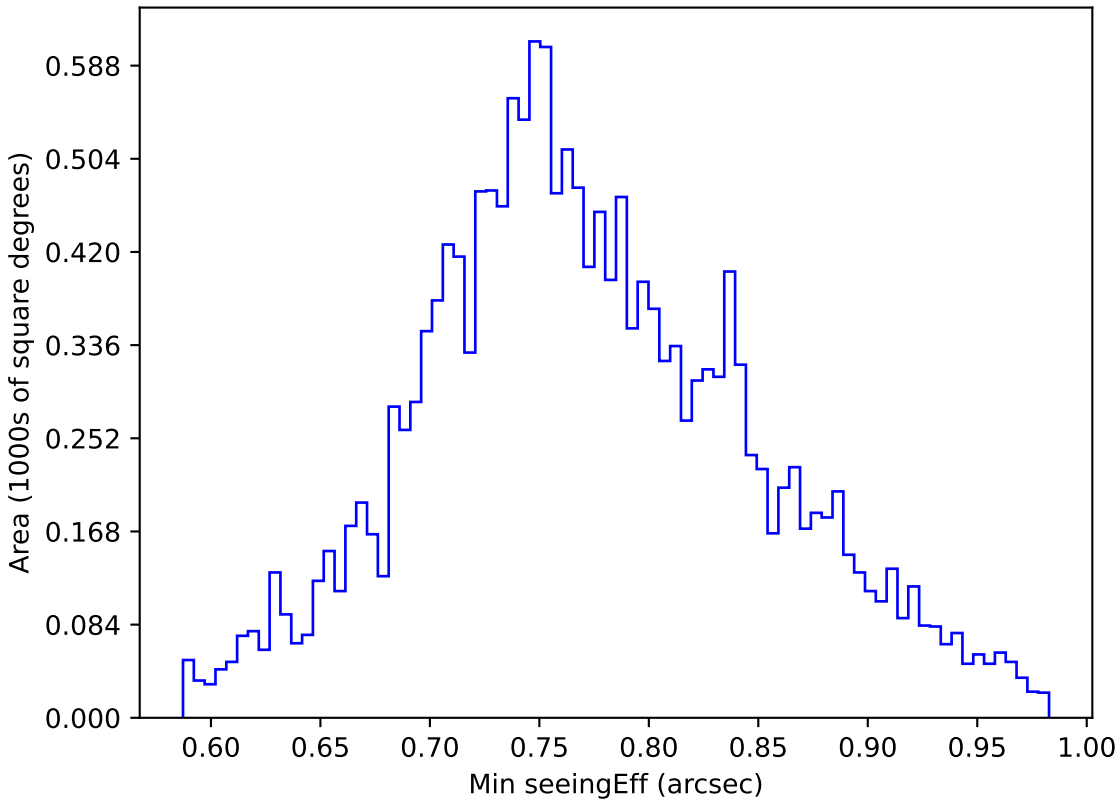
ddf_acor_sf10_lsf20_lsr50_v3.4_10yrs WFD u band: Min seeingEff
