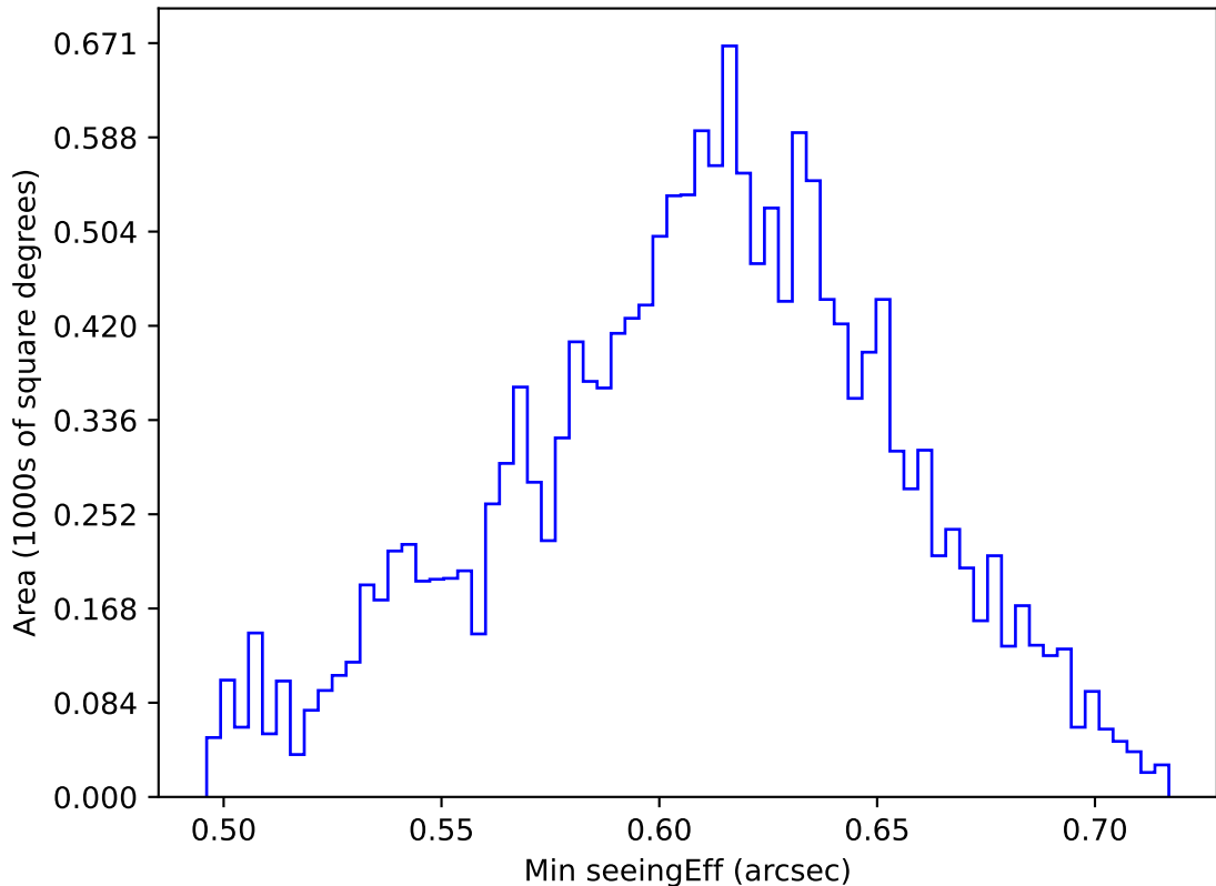
ddf_acor_sf10_lsf20_lsr50_v3.4_10yrs WFD r band: Min seeingEff
