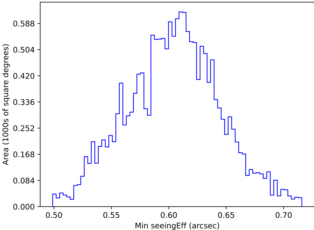
ddf_acor_sf10_lsf20_lsr50_v3.4_10yrs WFD i band: Min seeingEff
