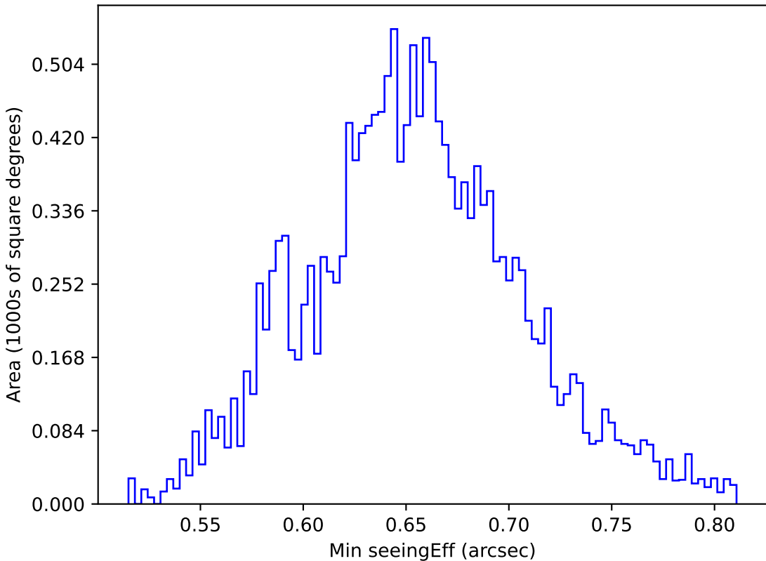
ddf_acor_sf10_lsf20_lsr50_v3.4_10yrs WFD g band: Min seeingEff
