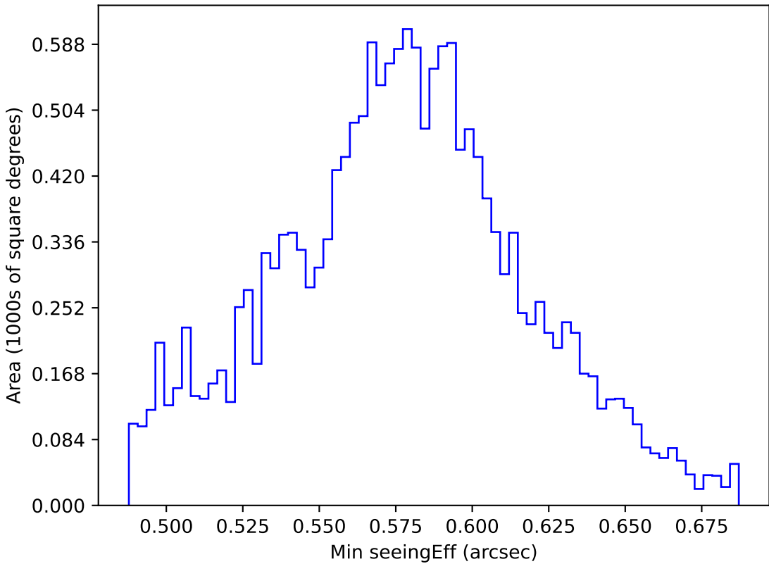
ddf_acor_sf10_lsf20_lsr50_v3.4_10yrs WFD all bands: Min seeingEff
