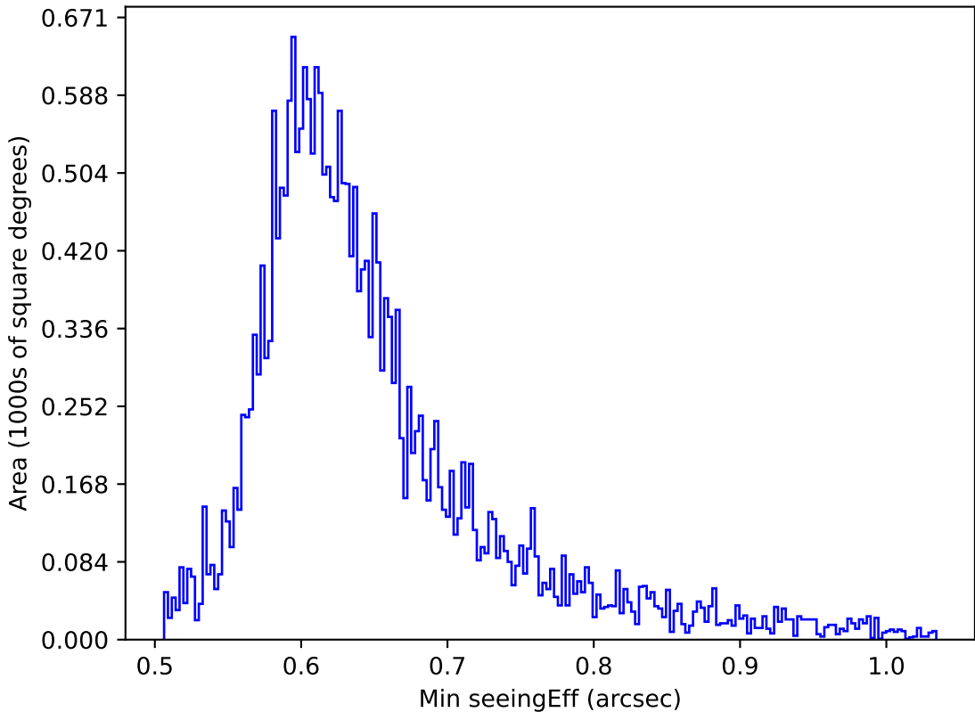
ddf_acor_sf10_lsf20_lsr50_v3.4_10yrs All sky z band: Min seeingEff
