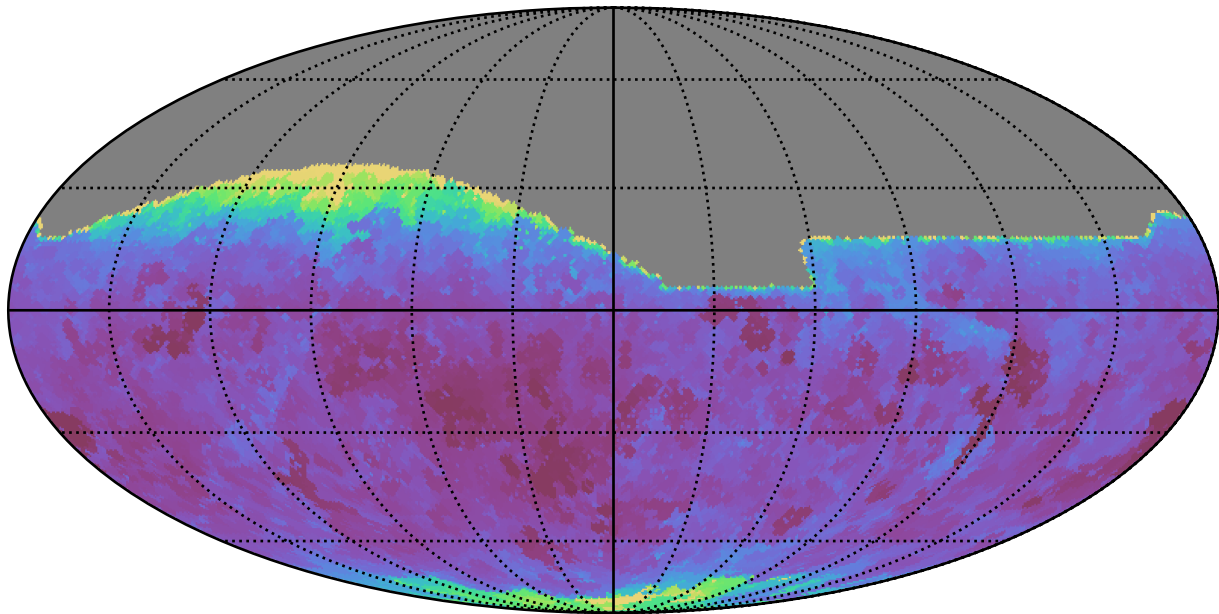
ddf_acor_sf10_lsf20_lsr50_v3.4_10yrs All sky r band: Min seeingEff
