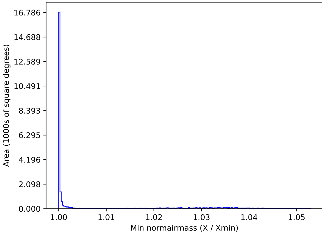
ddf_acor_sf10_lsf20_lsr50_v3.4_10yrs All sky g band: Min normairmass
