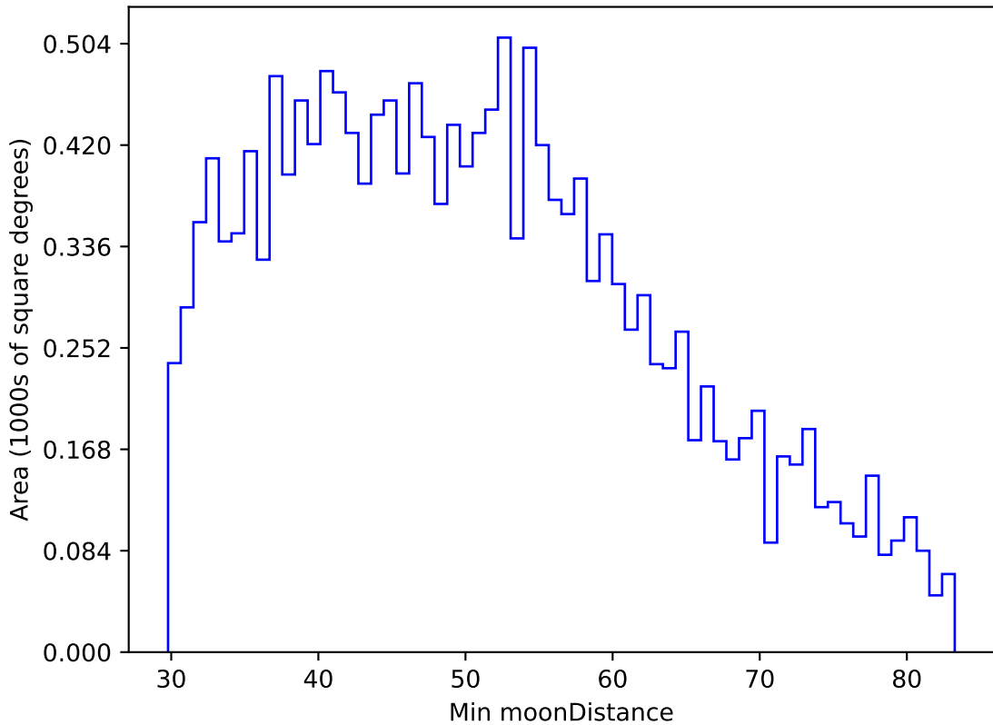
ddf_acor_sf10_lsf20_lsr50_v3.4_10yrs WFD u band: Min moonDistance
