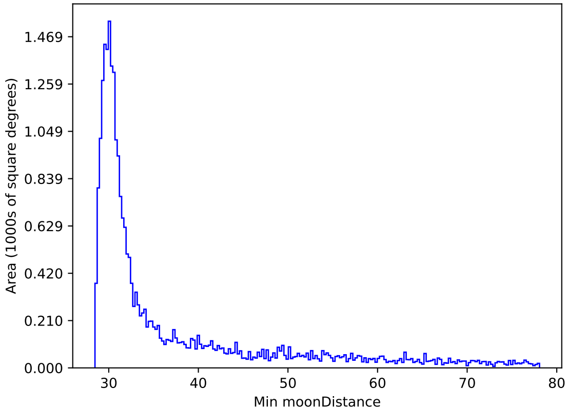
ddf_acor_sf10_lsf20_lsr50_v3.4_10yrs All sky i band: Min moonDistance
