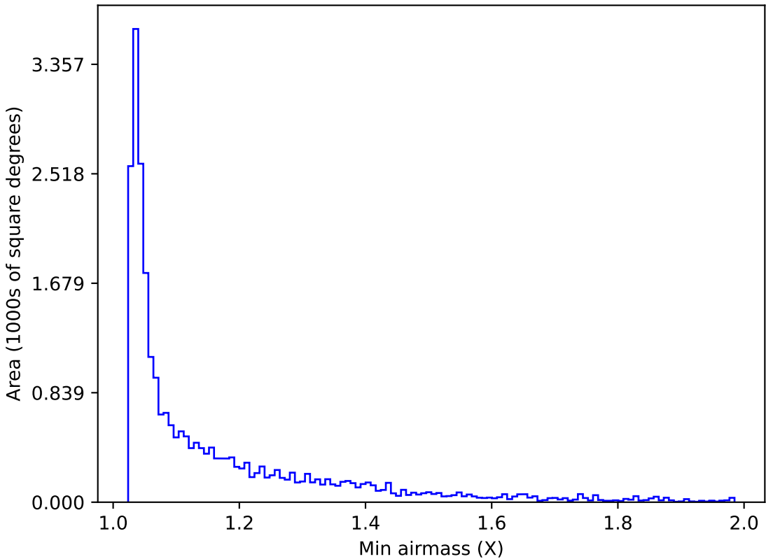
ddf_acor_sf10_lsf20_lsr50_v3.4_10yrs Yr 1 i band: Min airmass
