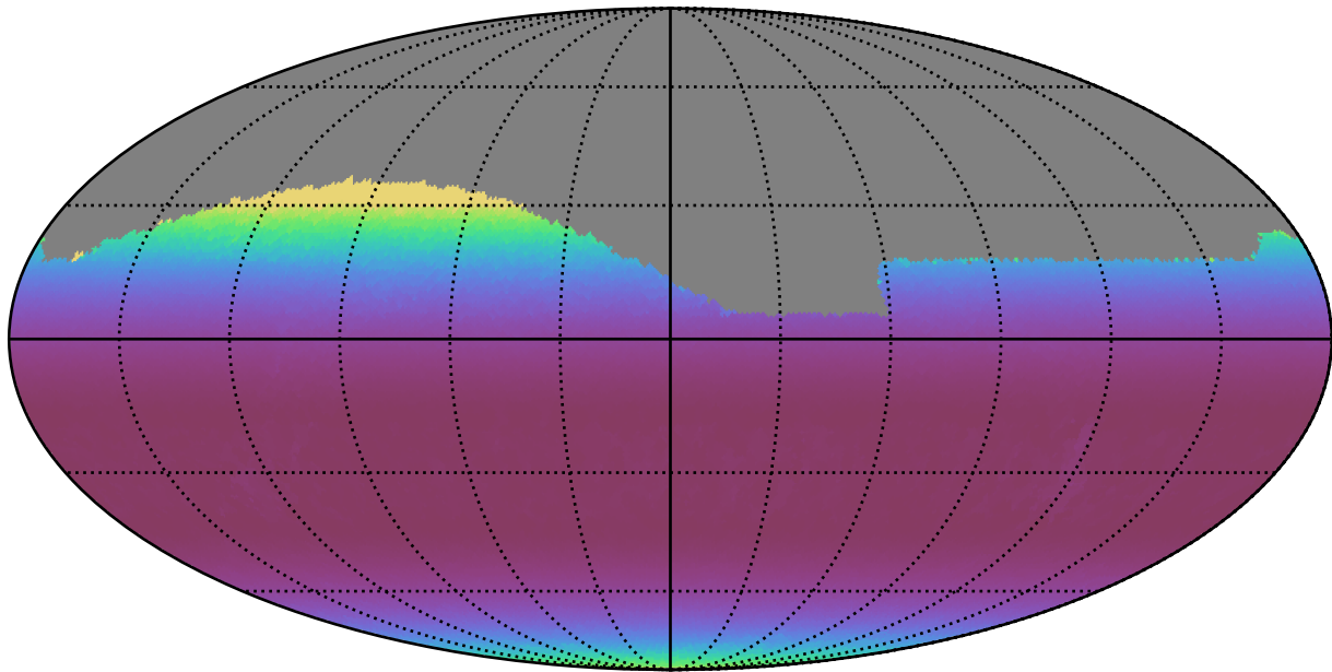
ddf_acor_sf10_lsf20_lsr50_v3.4_10yrs Yr 1 all bands: Min airmass
