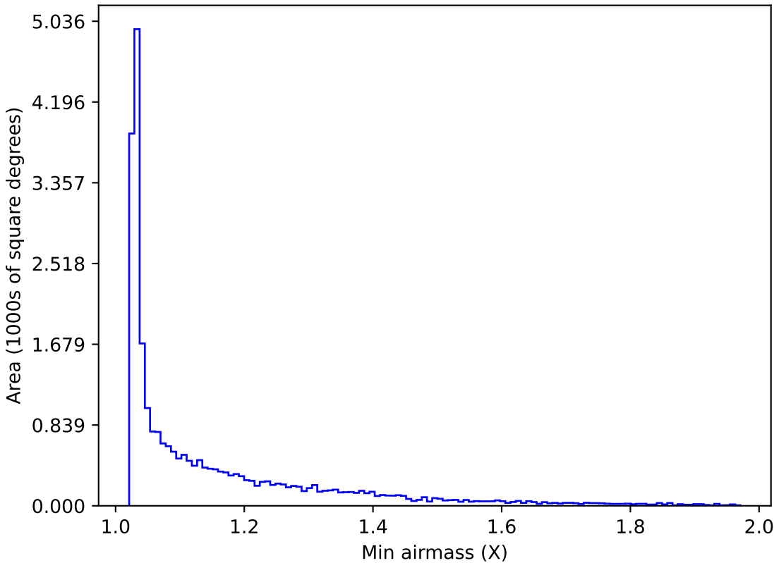
ddf_acor_sf10_lsf20_lsr50_v3.4_10yrs Yr 1 all bands: Min airmass
