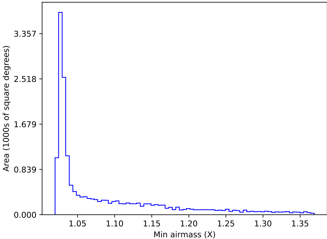
ddf_acor_sf10_lsf20_lsr50_v3.4_10yrs WFD z band: Min airmass
