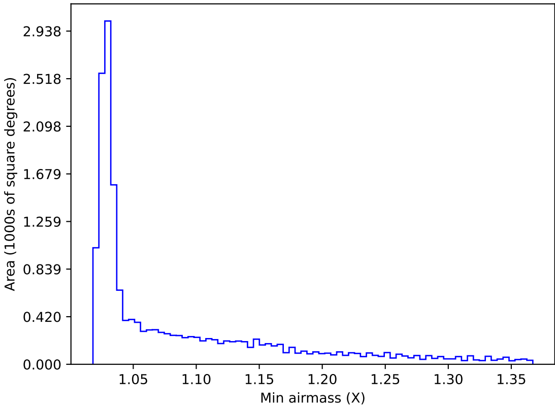
ddf_acor_sf10_lsf20_lsr50_v3.4_10yrs WFD i band: Min airmass
