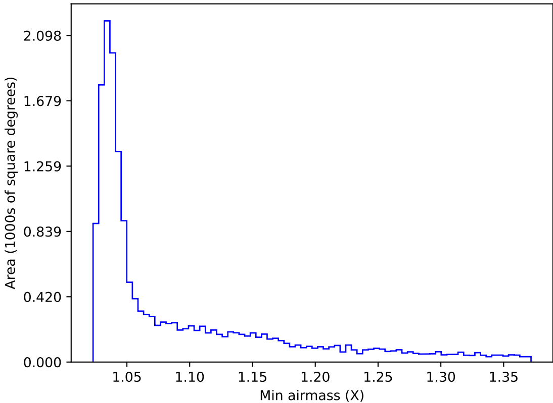
ddf_acor_sf10_lsf20_lsr50_v3.4_10yrs WFD g band: Min airmass
