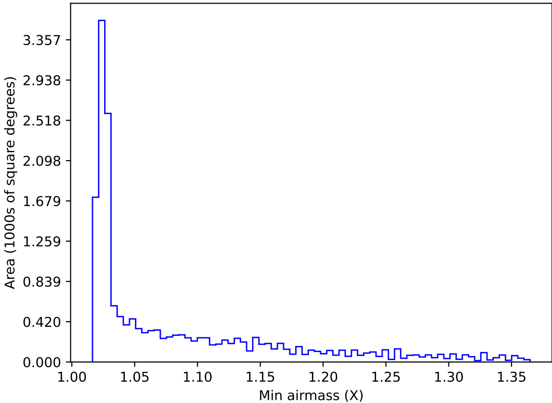
ddf_acor_sf10_lsf20_lsr50_v3.4_10yrs WFD all bands: Min airmass
