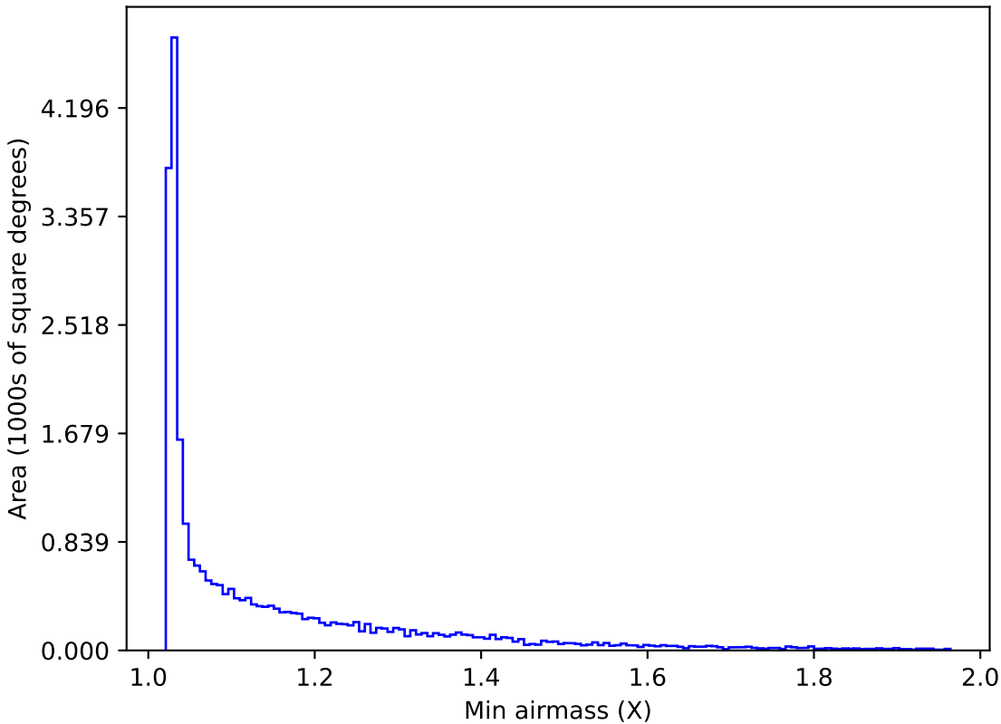
ddf_acor_sf10_lsf20_lsr50_v3.4_10yrs All sky z band: Min airmass
