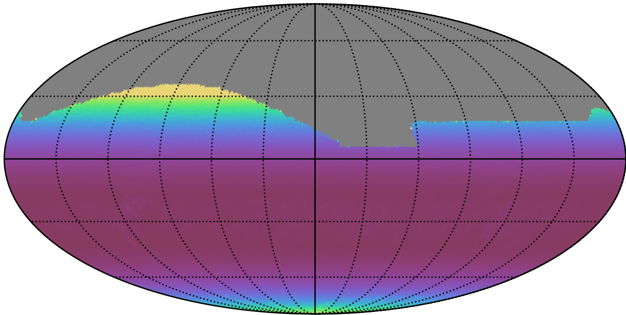
ddf_acor_sf10_lsf20_lsr50_v3.4_10yrs All sky r band: Min airmass
