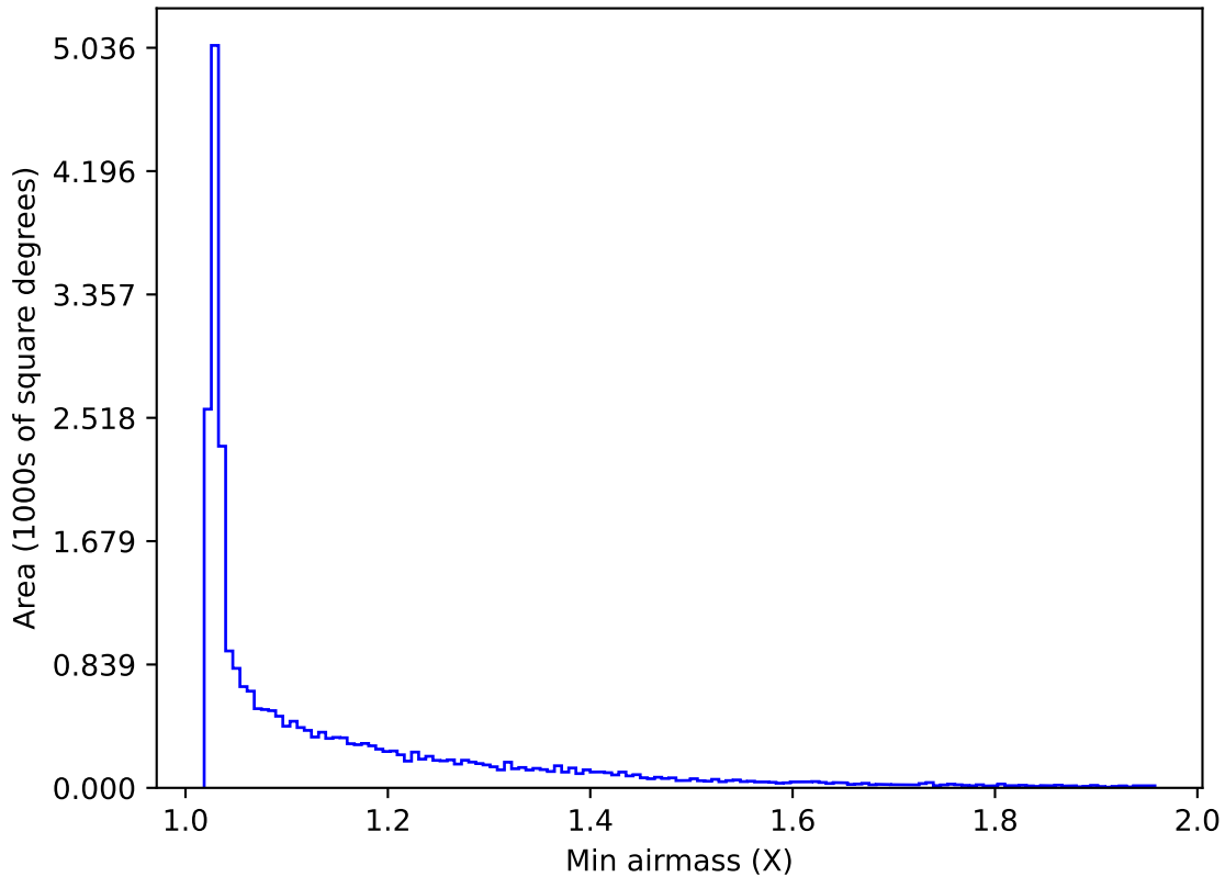
ddf_acor_sf10_lsf20_lsr50_v3.4_10yrs All sky i band: Min airmass
