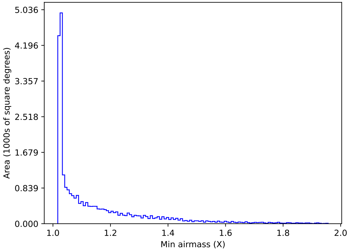
ddf_acor_sf10_lsf20_lsr50_v3.4_10yrs All sky all bands: Min airmass
