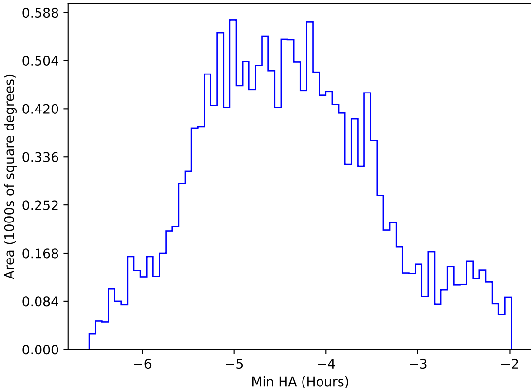
ddf_acor_sf10_lsf20_lsr50_v3.4_10yrs WFD z band: Min HA
